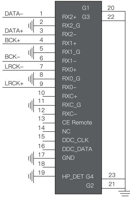
Figure 2: HDMI I2S Input Diagram
